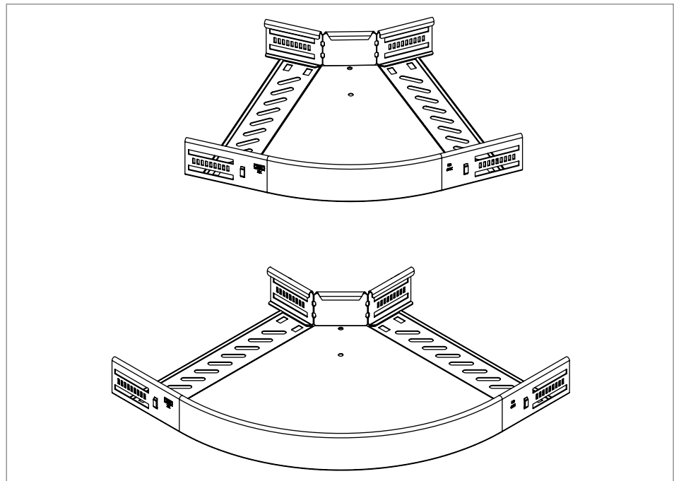
Fig. 3: 45° and 90° bends
