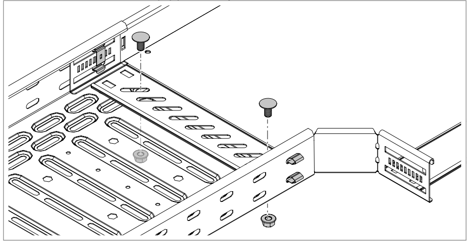
Fig. 52: Screwing on the joint plate
