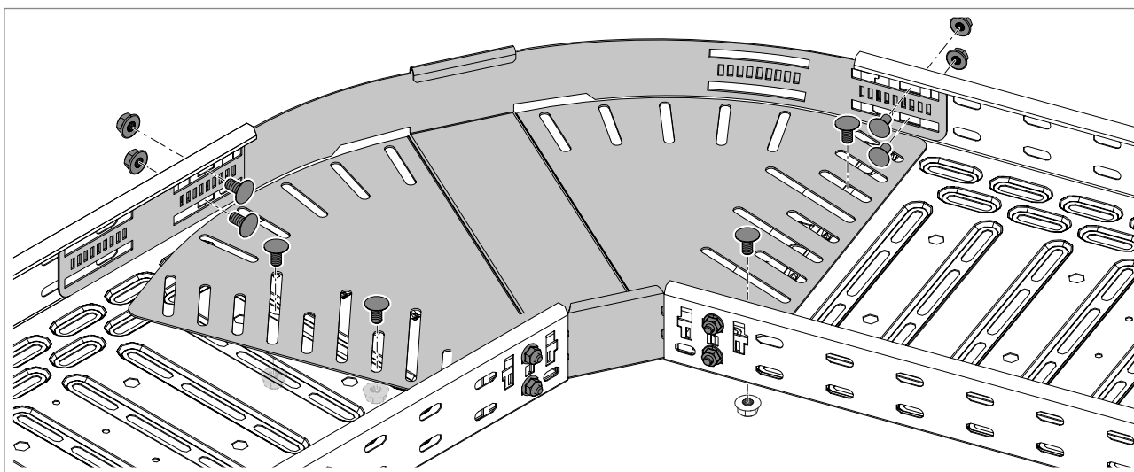
Abb. 66: Screwing connector and joint plate to trays
