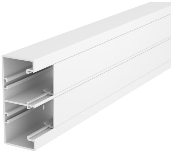
Trunking base and cover with base perforation for direct wall mounting.
